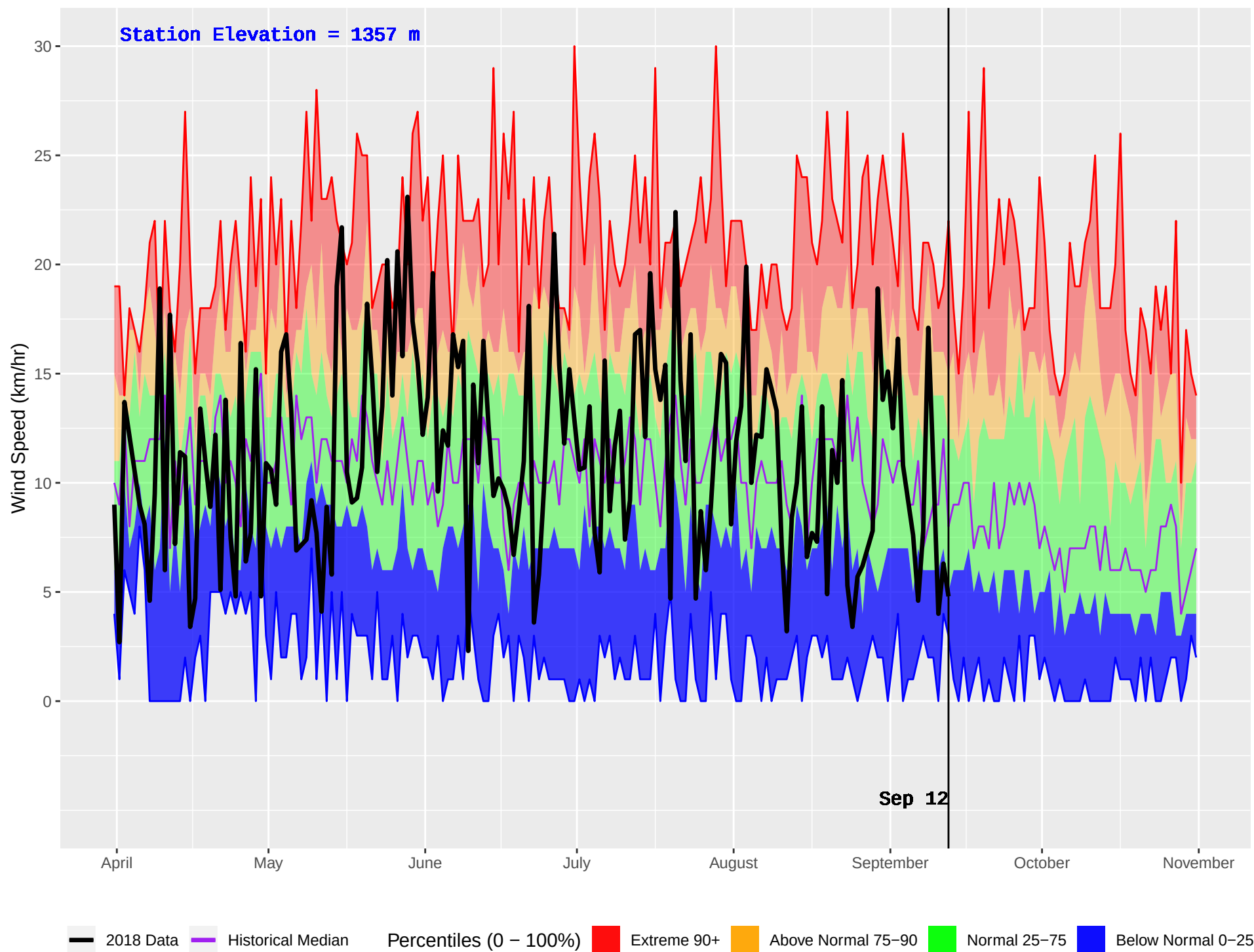
WHITE RIVER (790) : Historical (1989–2016) and Current (2018) Daily Wind Speed
