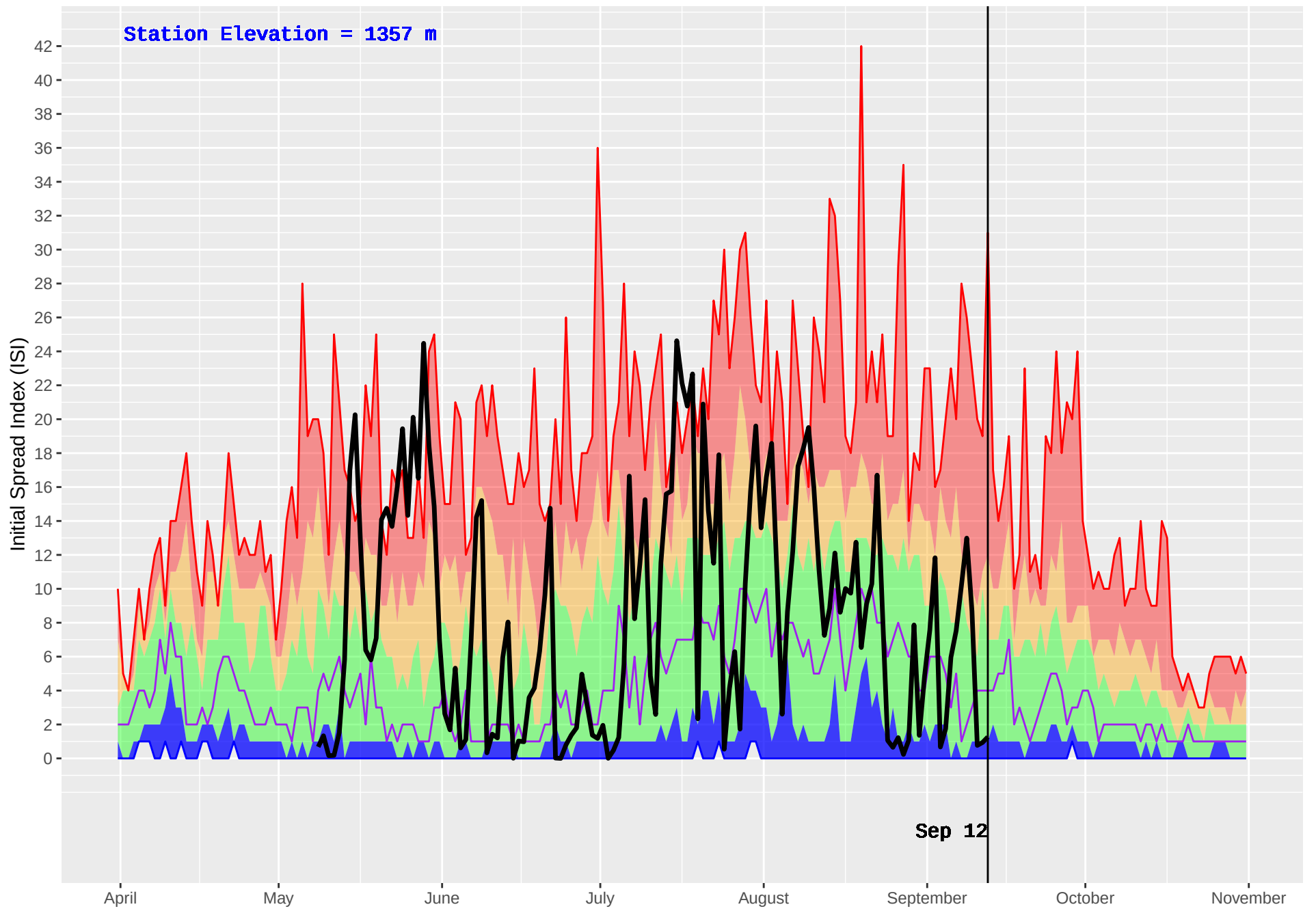
WHITE RIVER (790) : Historical (1989–2016) and Current (2018) Daily Initial Spread Index (ISI)
